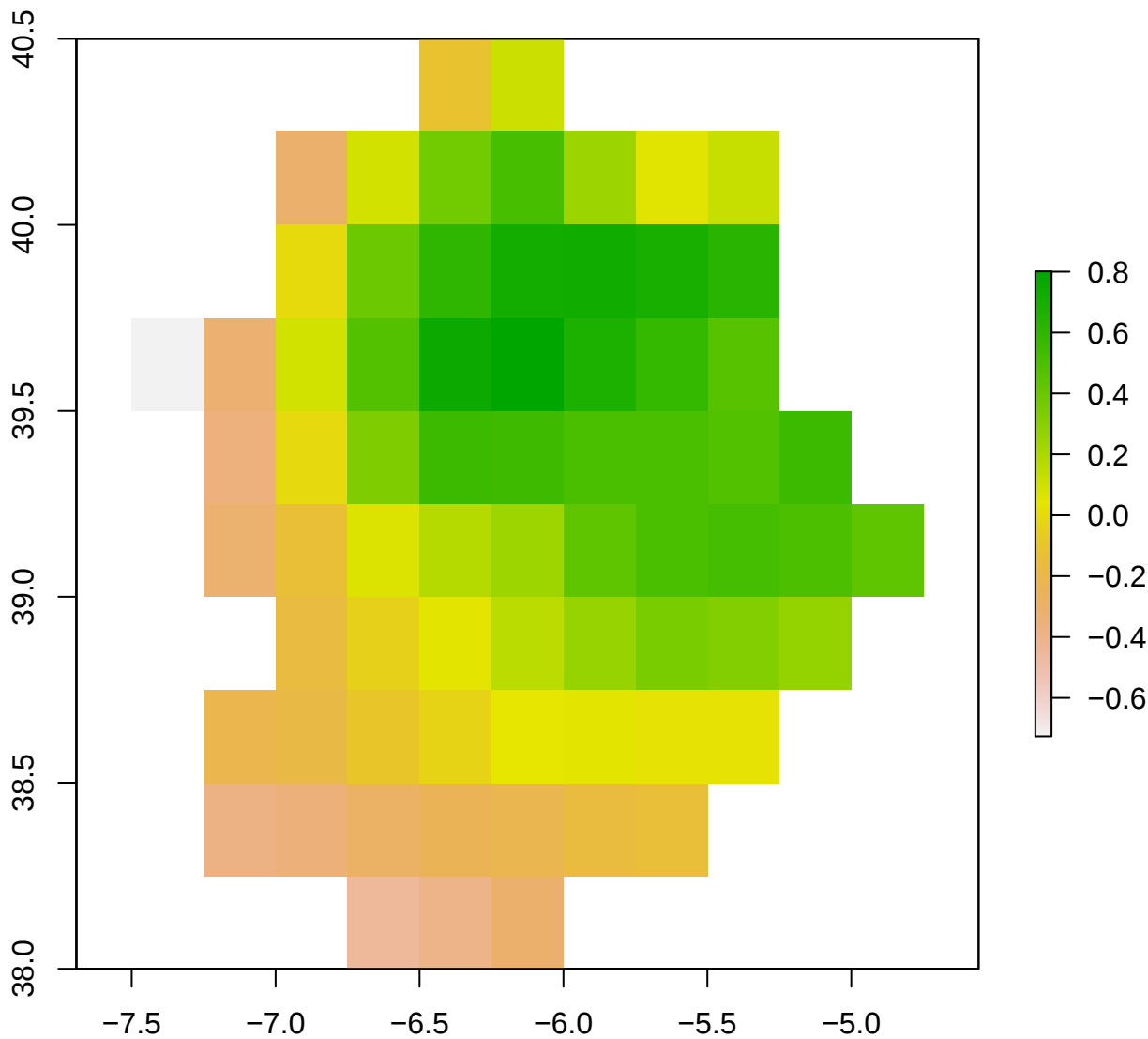
spi12_month - ES43 2004-11-01
