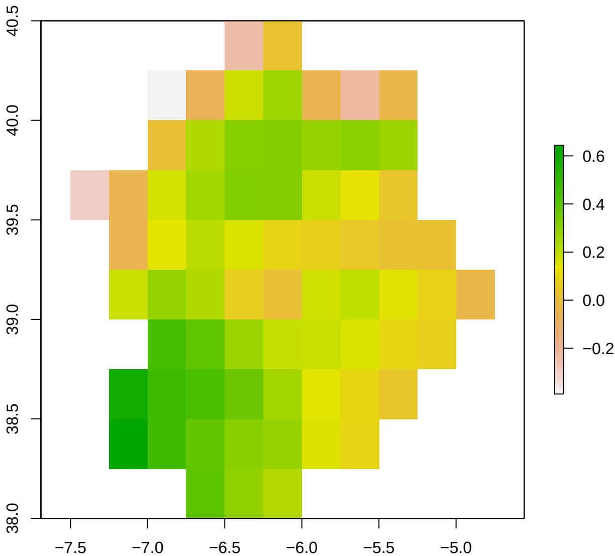
spi12_month - ES43 2004-02-01
