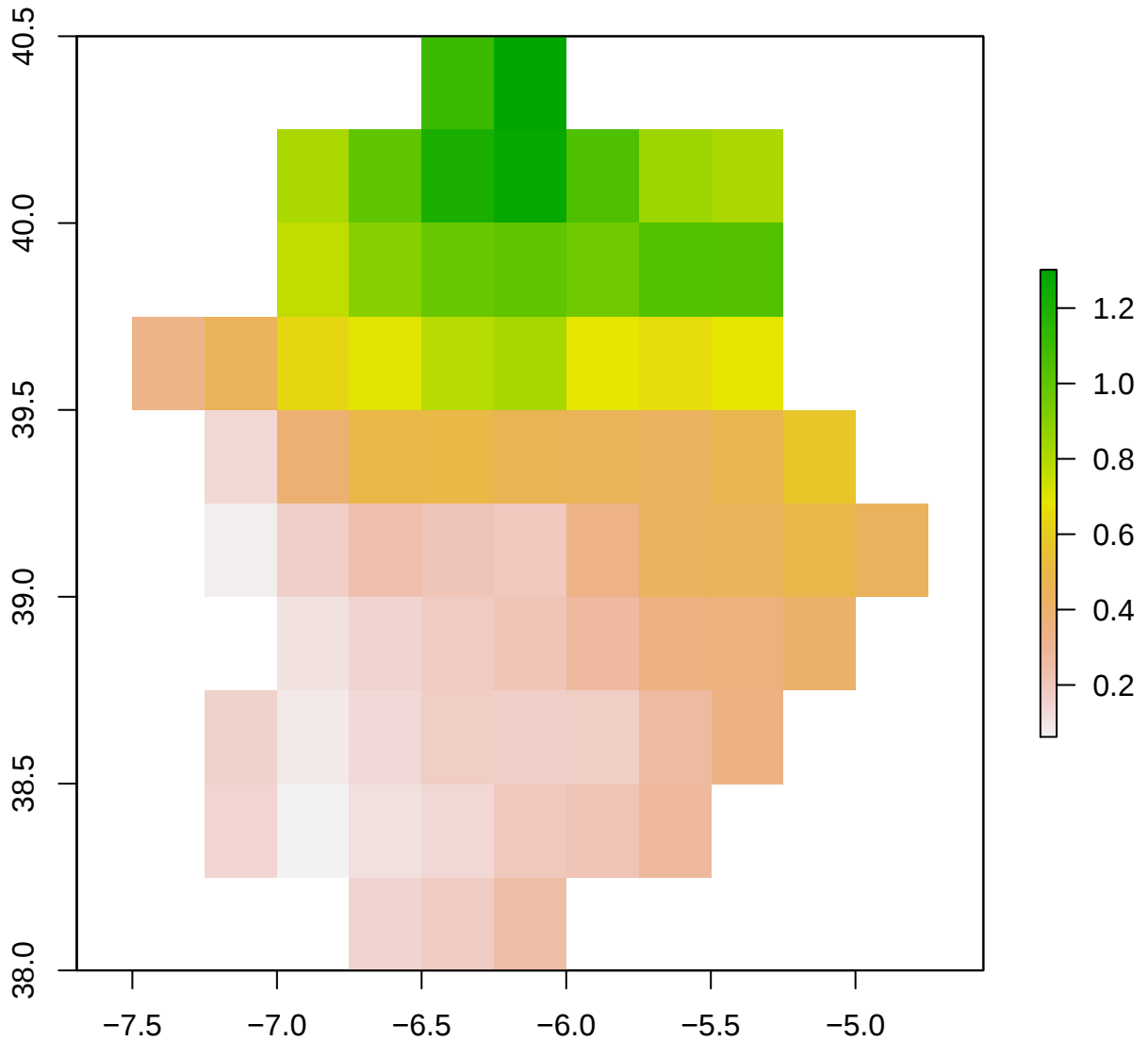
spi12_month - ES43 2003-03-01
