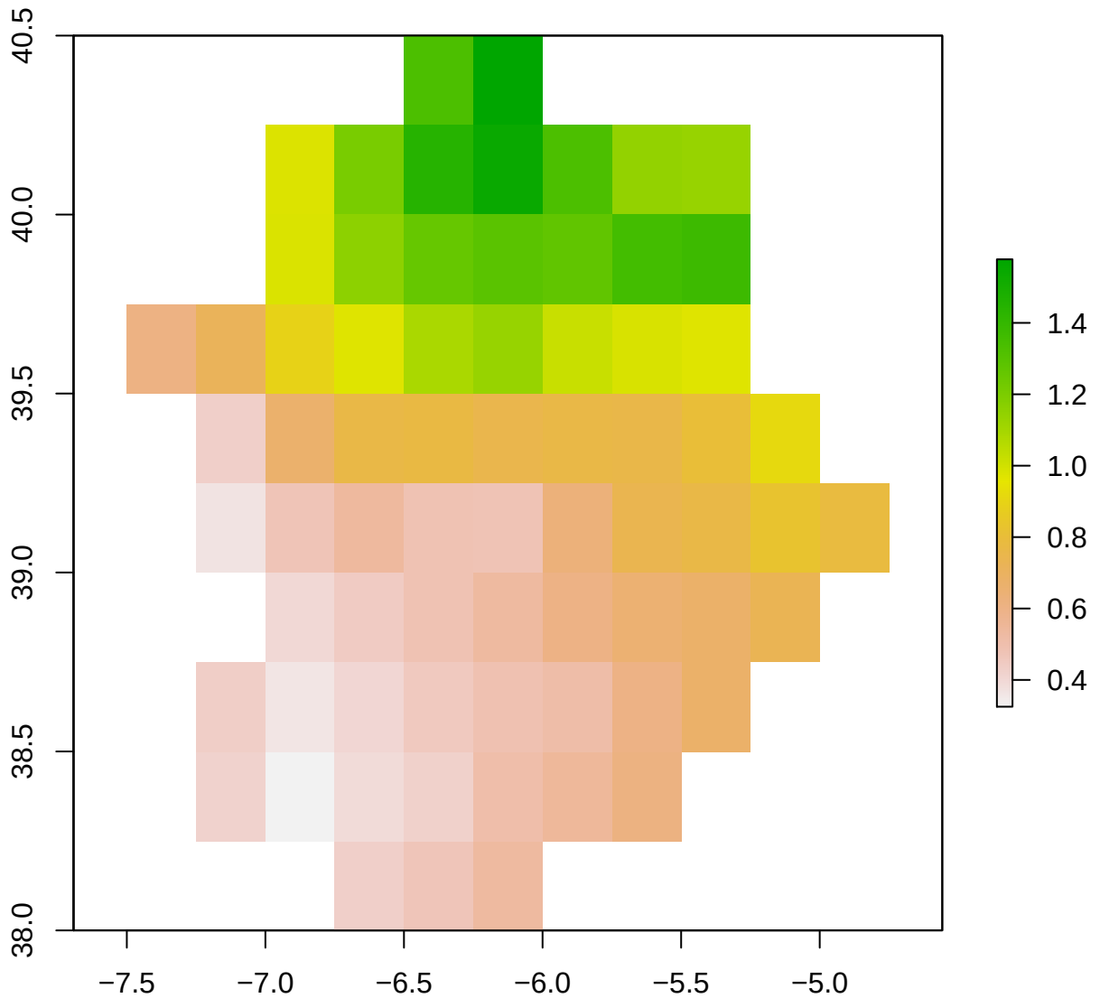
spi12_month - ES43 2003-02-01
