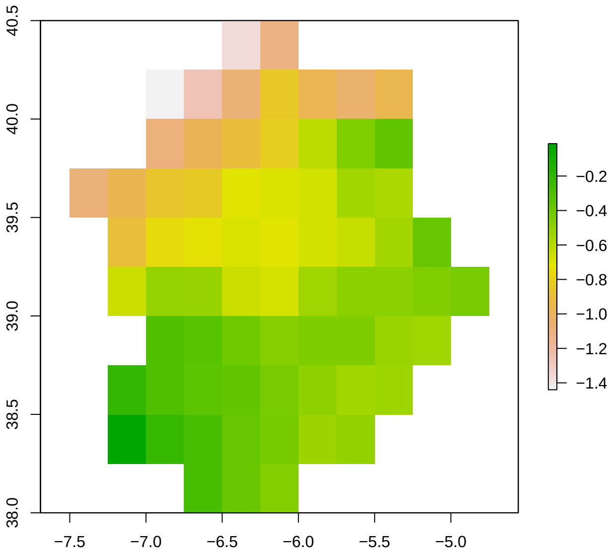
spi12_month - ES43 2002-07-01
