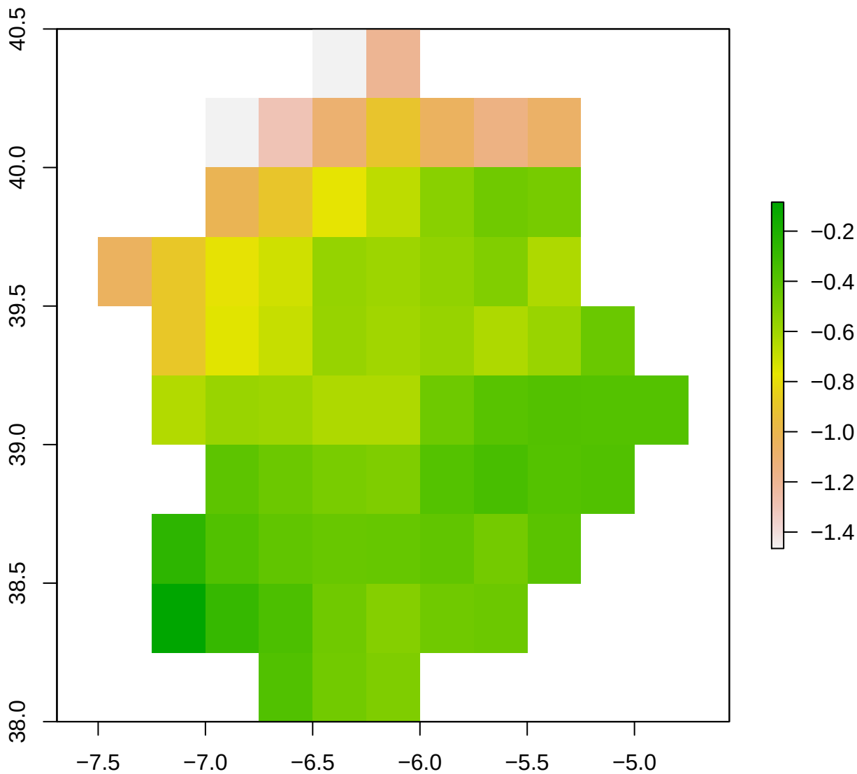
spi12_month - ES43 2002-02-01
