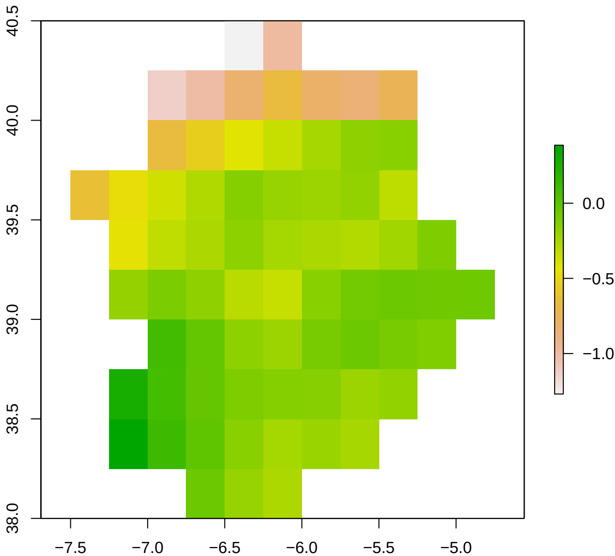
spi12_month - ES43 2002-01-01
