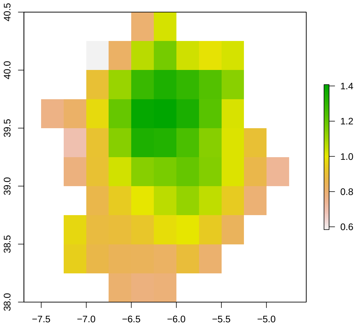
spi12_month - ES43 2001-07-01
