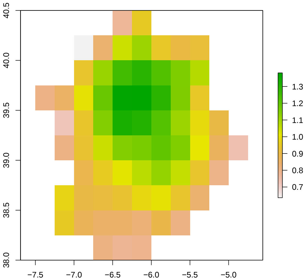
spi12_month - ES43 2001-06-01
