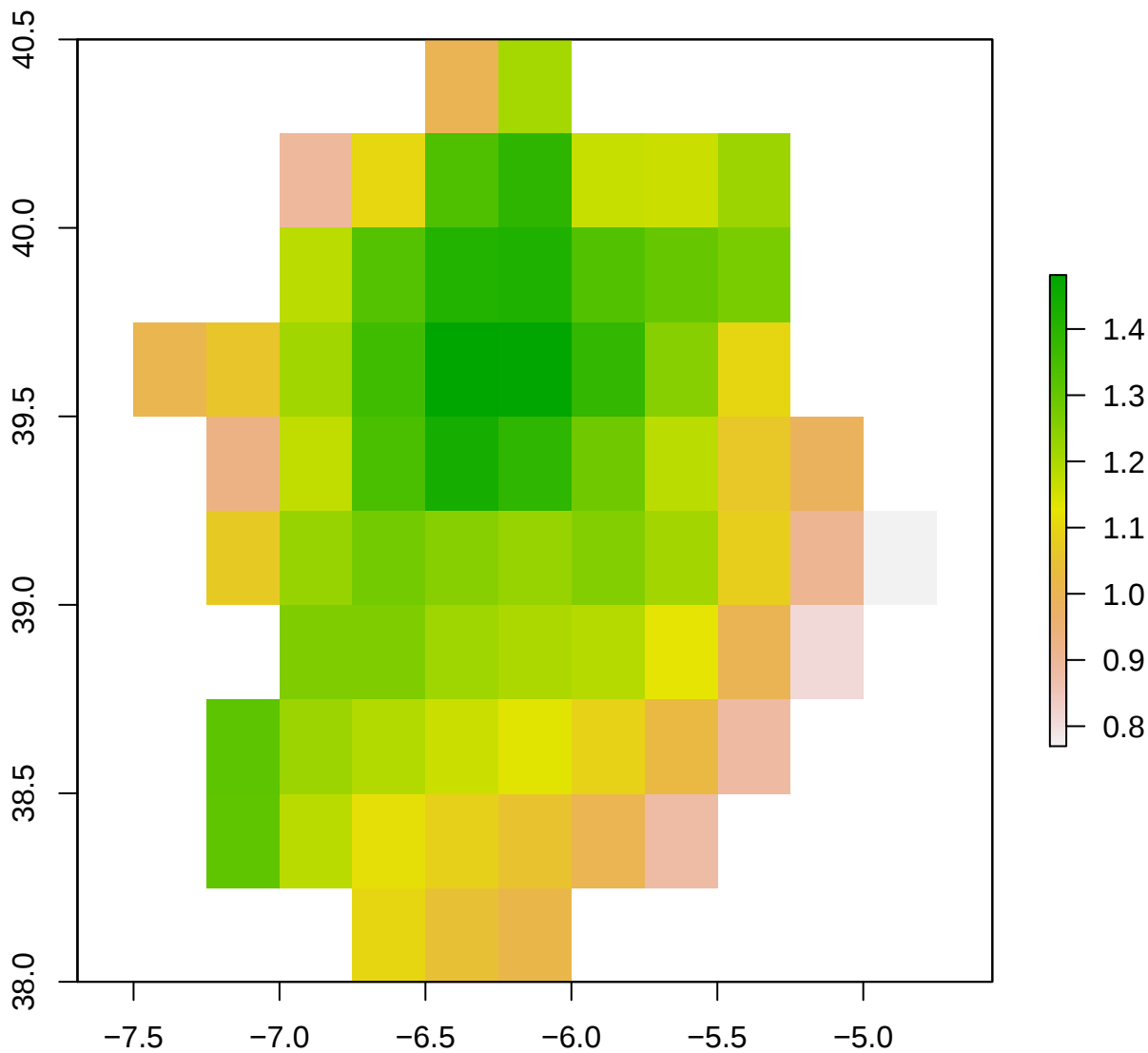
spi12_month - ES43 2001-04-01
